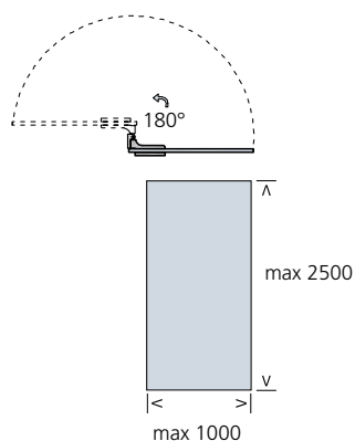
Porta singola vetro-muro Single door wall to glass
