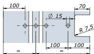
Contro per art. 280A (Alimentazione 6-12 Vac/Vad 0.5-0.8 A) Electric lock keeper for art. 280A (Power supply 6-12 Vac/Vad 0.5-0.8 A)
